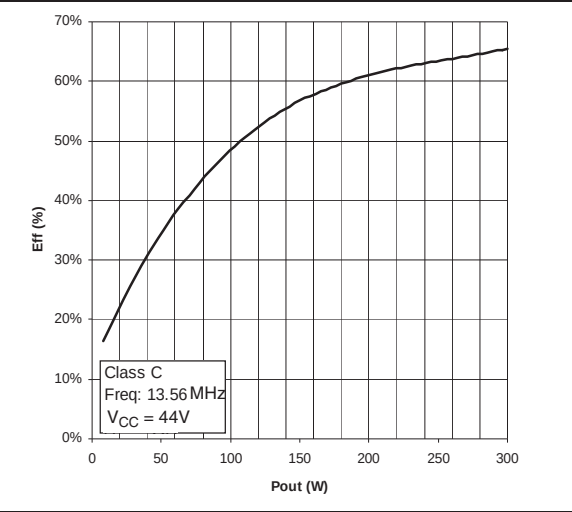
Figure 4. Efficiency vs POUT
